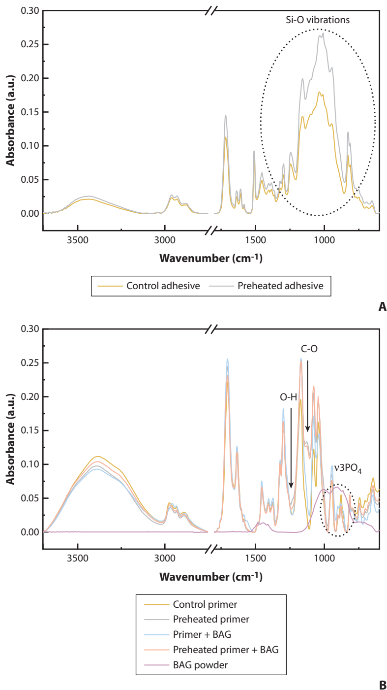
Figure 2. ATR-FTIR spectra of different modes of use, A, Bonding agent, B, Primer. ATR-FTIR, Attenuated total reflection Fourier transform infrared spectroscopy; BAG, Bioglass 45S5.
