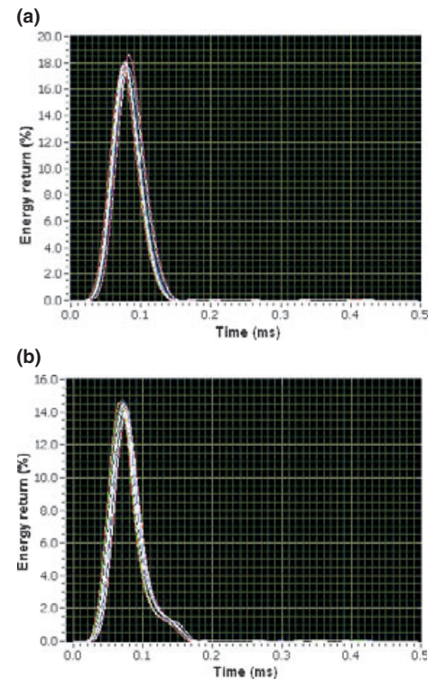
Fig. 3. Examples of energy return graphs generated by the Perimeter® software. Zirconia abutment with composite resin onlay, corresponding LC of 0.0498 (a); Composite resin abutment with composite resin onlay, corresponding LC of 0.0679 (b).
