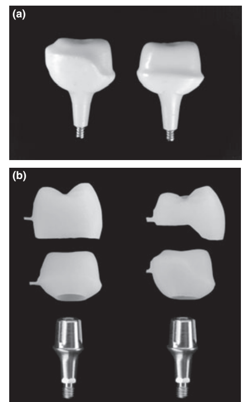
Fig. 1. Original zirconia abutments provided by the manufacturer (a, onlay design on left, crown design on right). Composite resin abutments resulting from the assembly of a solid abutment (b, bottom), the composite mesostructure (b, middle) and the corresponding restorations (b, top).
