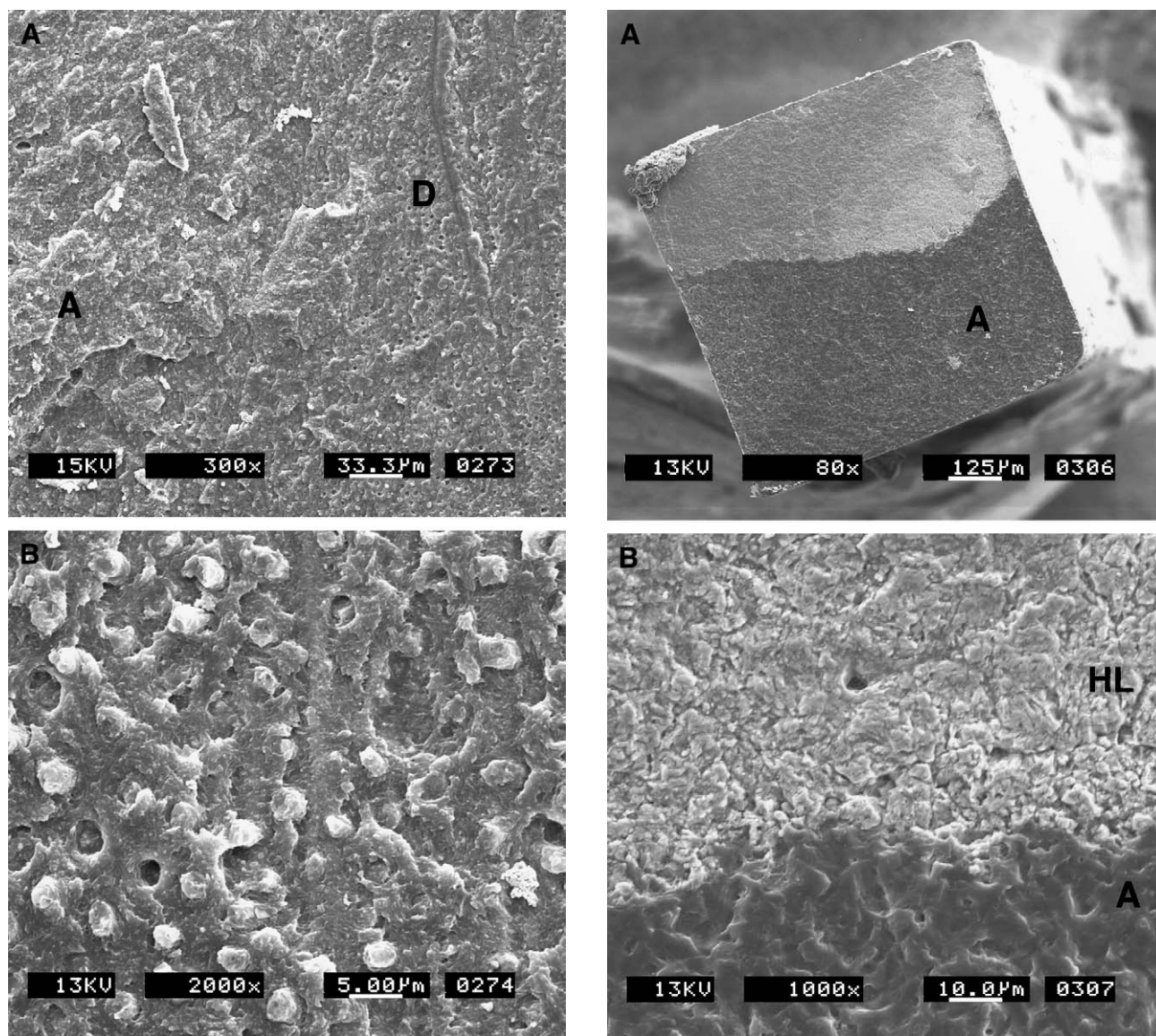
Fig. 4. A , Typical SEM micrograph of fractured beam from IDS group, which failed at 57.4 MPa. Note mixed interfacial failure, mainly in dentin ( D ) and, in part, in filled adhesive ( A ). B , Higher magnification of dentin area on tooth side also suggests cohesive fracture in dentin beneath hybrid layer with blocked hybridized resin plugs. Original magnification \times 2000 .
